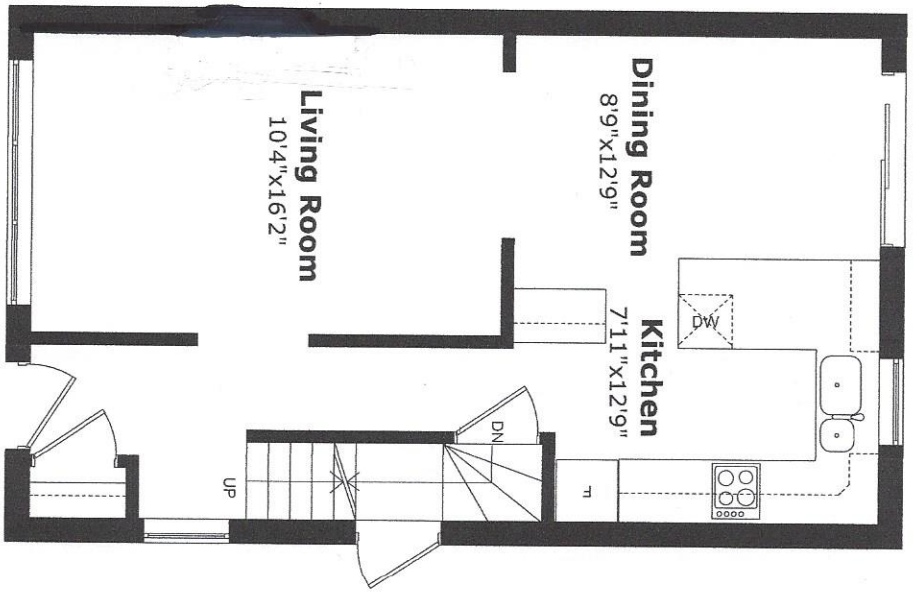
MAIN FLOOR
