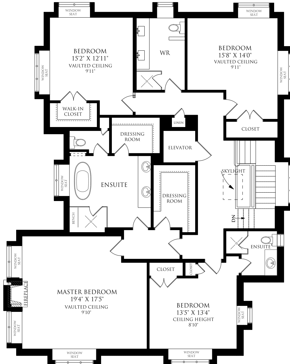
SECOND FLOOR 2062 SQUARE FEET
