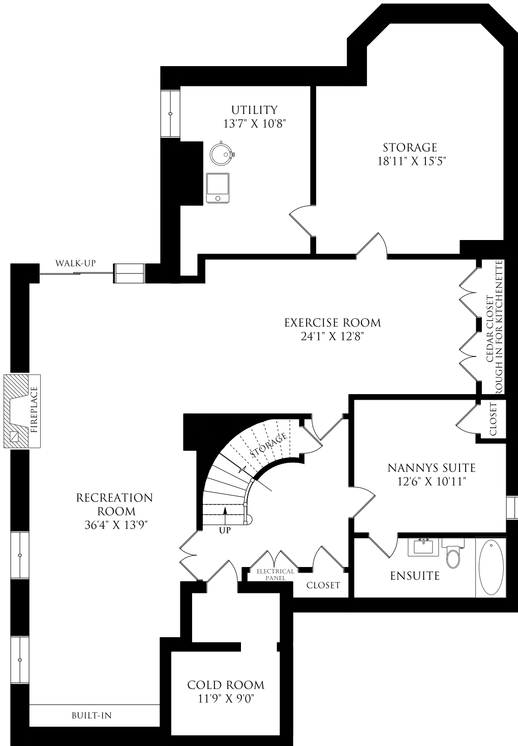
LOWER LEVEL 2000 SQUARE FEET
